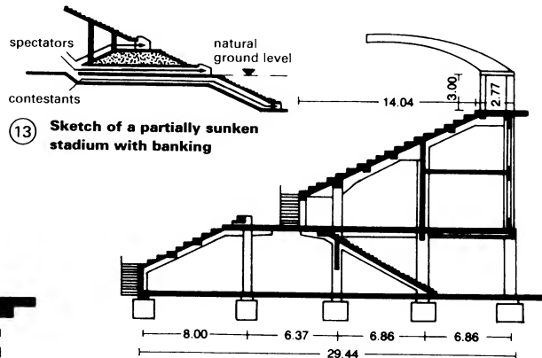
⑭ Section through the Vienna Stadium
